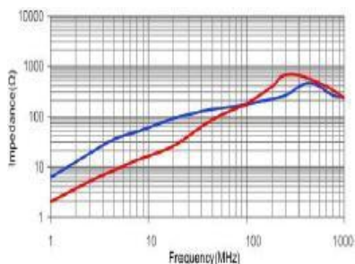
CMZ4520A-701TT
