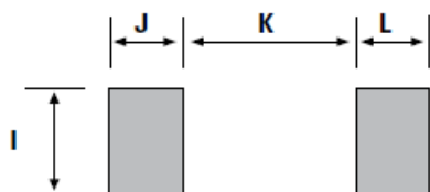
Mounting Pad Layout
